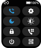
Status Bar
