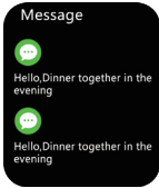
Notifications
