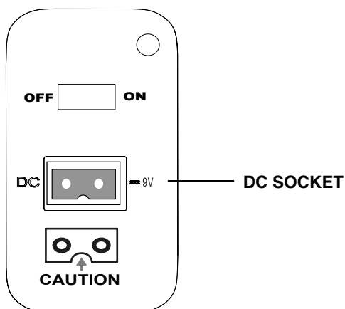
OPERATING PANEL
